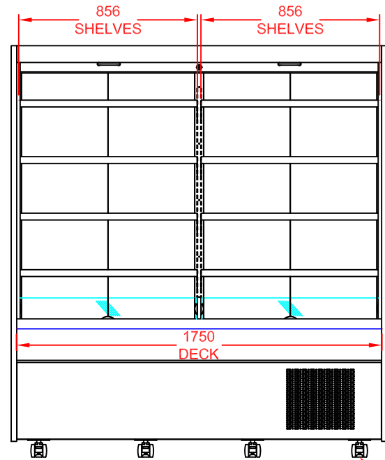
FRONT VIEW (CUSTOMER SIDE)
