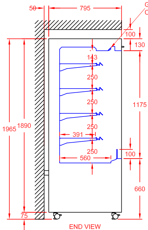
END VIEW
