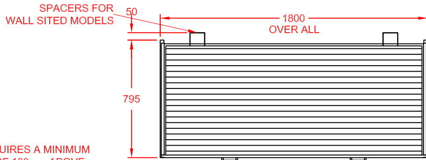
PLAN VIEW
