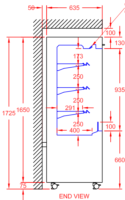
END VIEW
