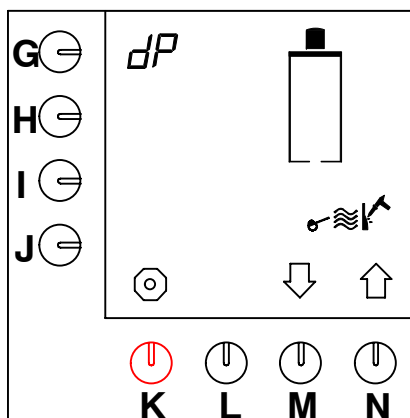
Fig. 18 Starting the descaling programme coffee-making system
