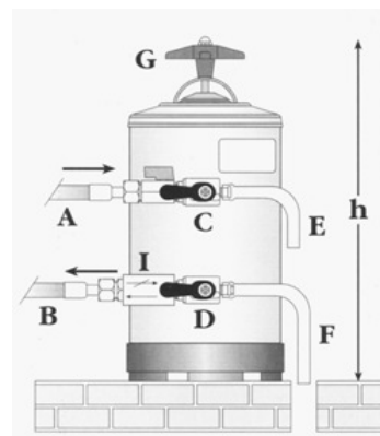
Fig 1: Installation Drawing
